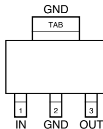
SOT-23 (S)
