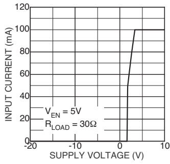
Input Current
